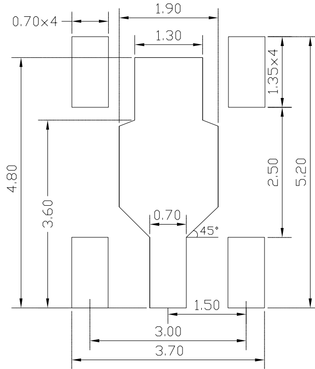
TYPICAL RECOMMENDED LAND PATTERN
