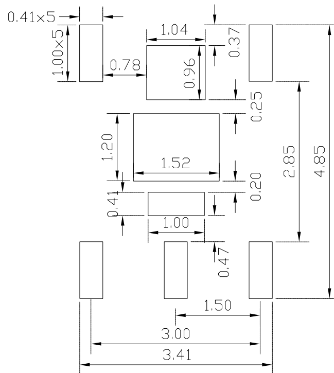
TYPICAL RECOMMENDED STENCIL
